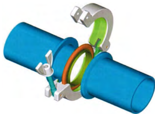
KF
